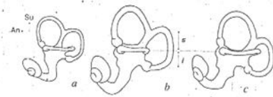
FIG. 2 Lateral aspect of the left labyrinths of a, Pan paniscus ; b, modern Homo sapiens ; and c, the Neanderthal cranium La Ferrassie 1. An, anterior; Su, superior. The sagittal labyrinthine index indicates what percentage of the posterior canal is situated inferiorly to the plane of the lateral canal ( l/s + 1 \times 100 ). Exact definitions and method of taking the measurements are given in refs 18, 20 and 21.
